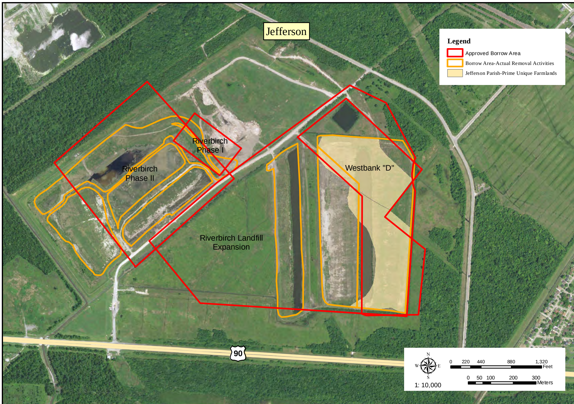
Borrow Map #6 Westbank "D", Riverbirch Phase I, Riverbirch Phase II and Riverbirch Landfill Expansion Borrow Sites - Jefferson Parish, LA
