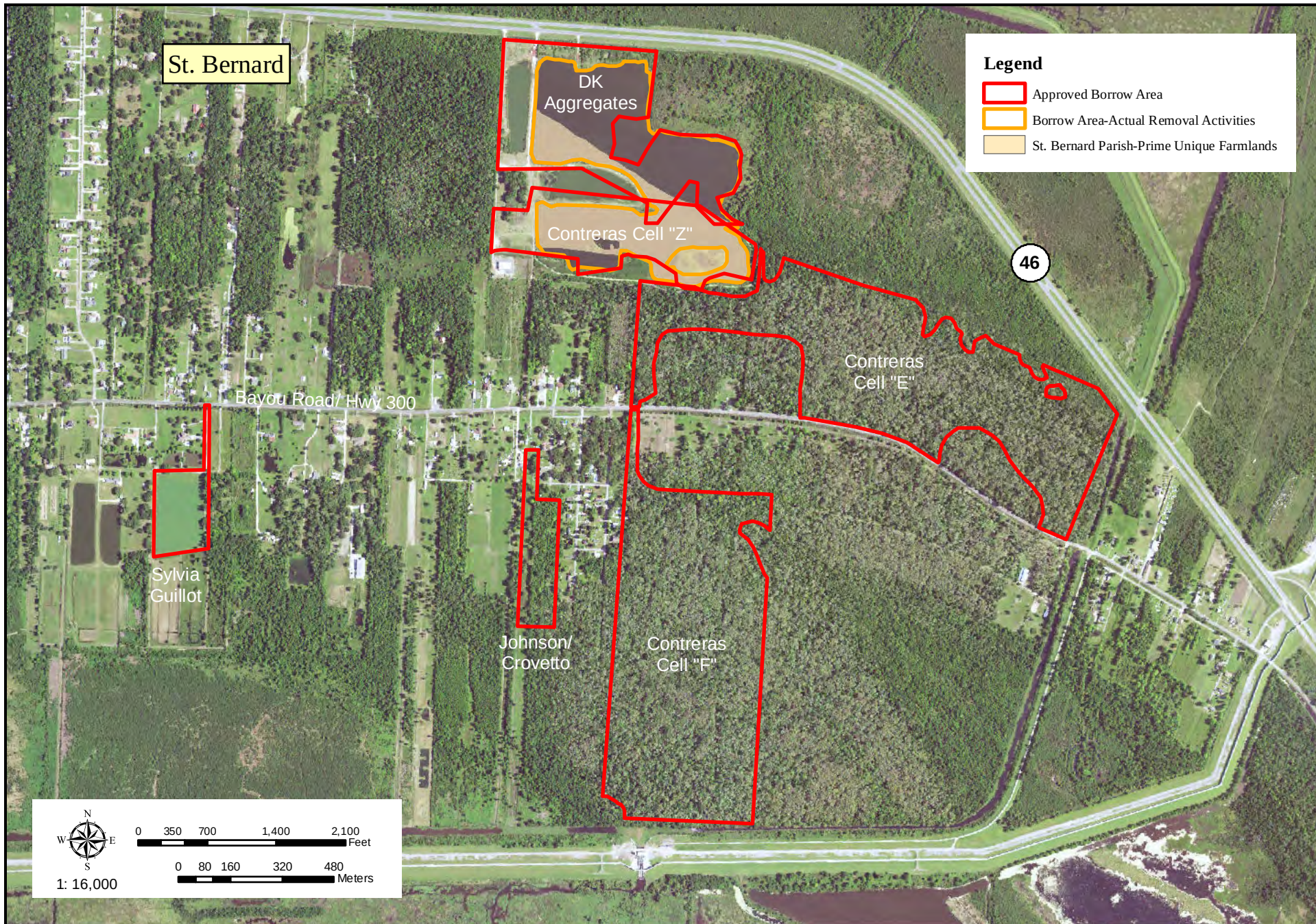
Borrow Map #24 Sylvia Guillot, Johnson/Crovetto, and DF Aggregates/Contreras Dirt Borrow Sites - St. Bernard Parish, LA
