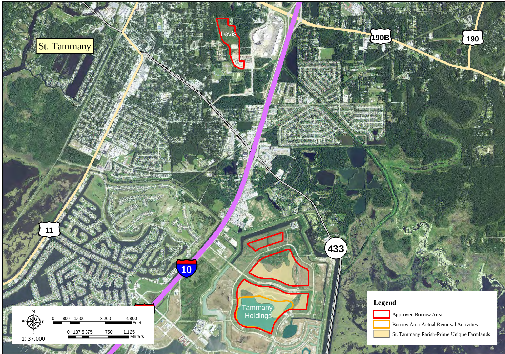
Borrow Map #31 Levis and Tammany Holding Borrow Sites - St. Tammany Parish, LA
