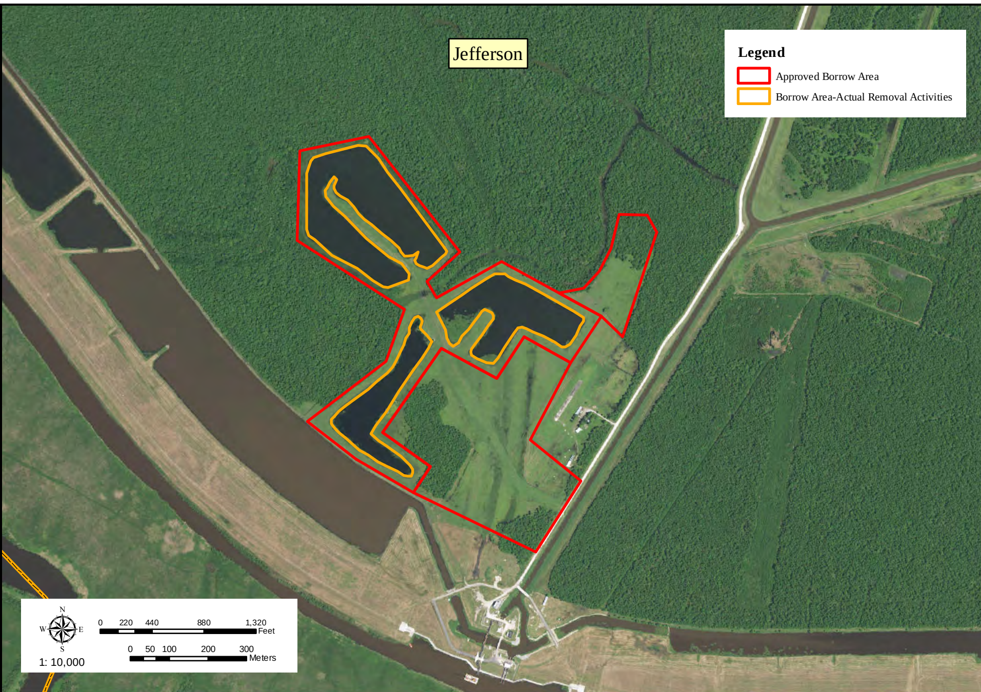
Borrow Map #8 Churchill Farms Phase I Borrow Site - Jefferson Parish, LA
