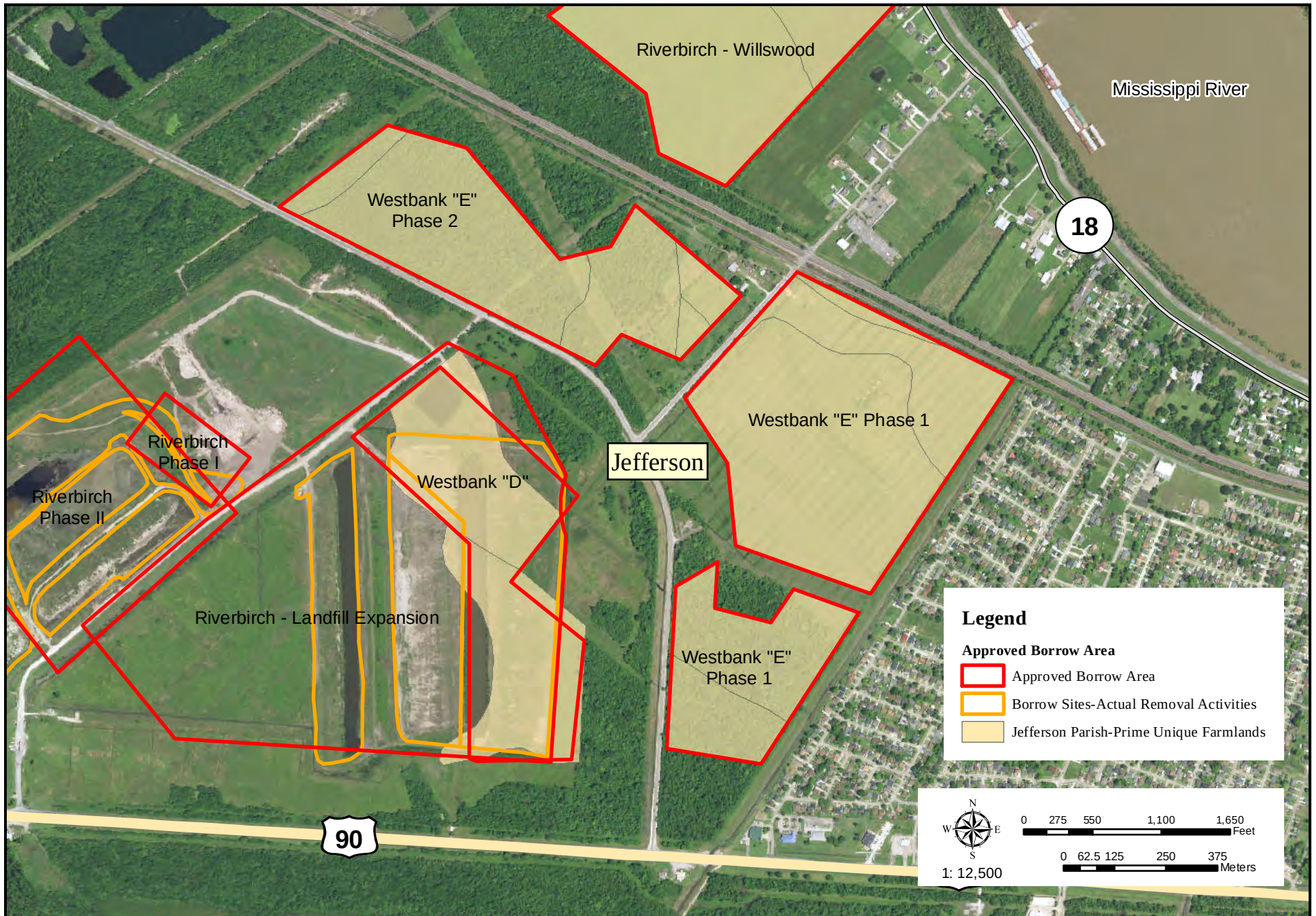
Borrow Map #5 Riverbirch Phase I, Riverbirch Phase II, Riverbirch Landfill Expansion, Riverbirch Willswood, Westbank "D" and Westbank "E" Borrow Sites - Jefferson Parish, LA
