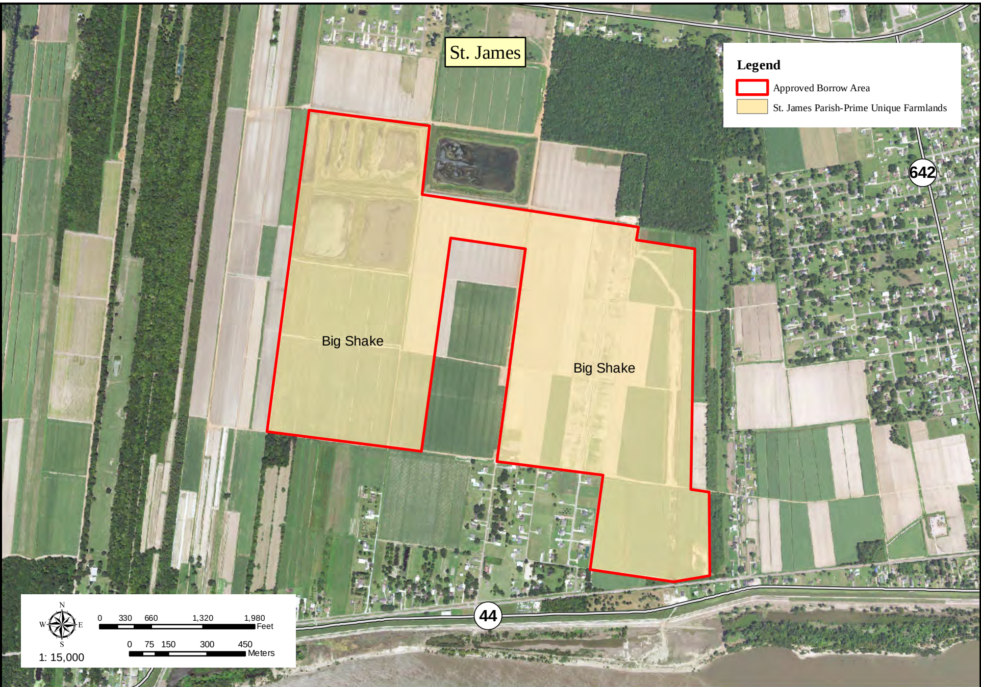
Borrow Map #29 Big Shake Borrow Site - St. James Parish, LA
