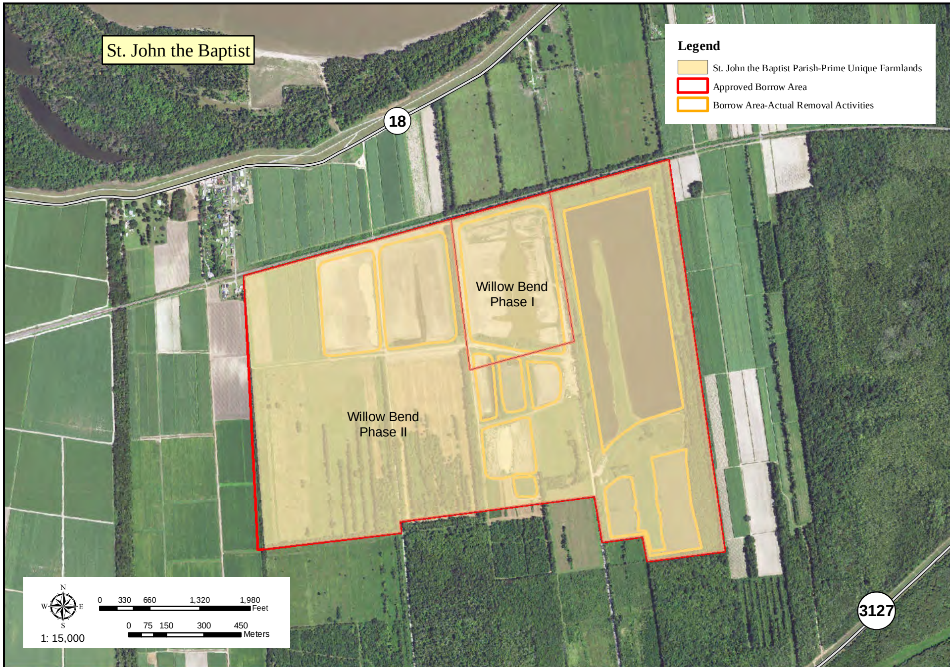
Borrow Map #30 Willow Bend and Willow Bend Phase 2 Borrow Site - St. John the Baptist Parish, LA
