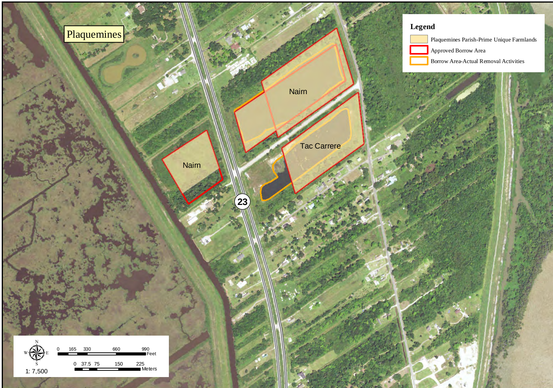
Borrow Map #20 Naim and Tac Carrere Borrow Sites - Plaquemines Parish, LA
